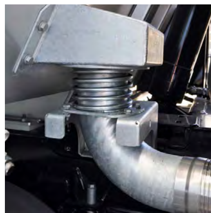
Tipper body heater
